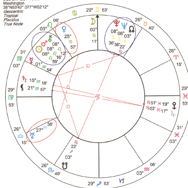
Chart 2 - Pluto/Neptune Conjunction
